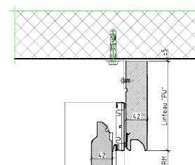
Faux linteau isolé "PU"
